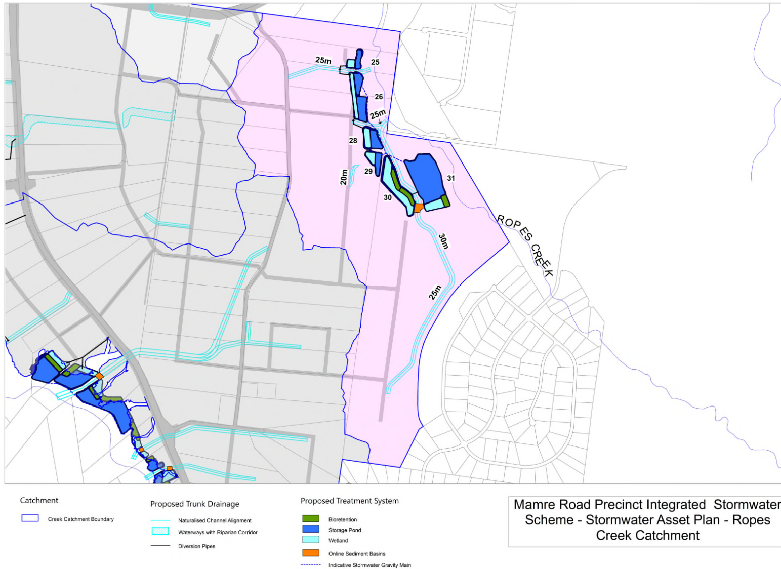
Figure 6.1.1 Stormwater assets in Mamre Road Precinct Ropes Creek catchment
