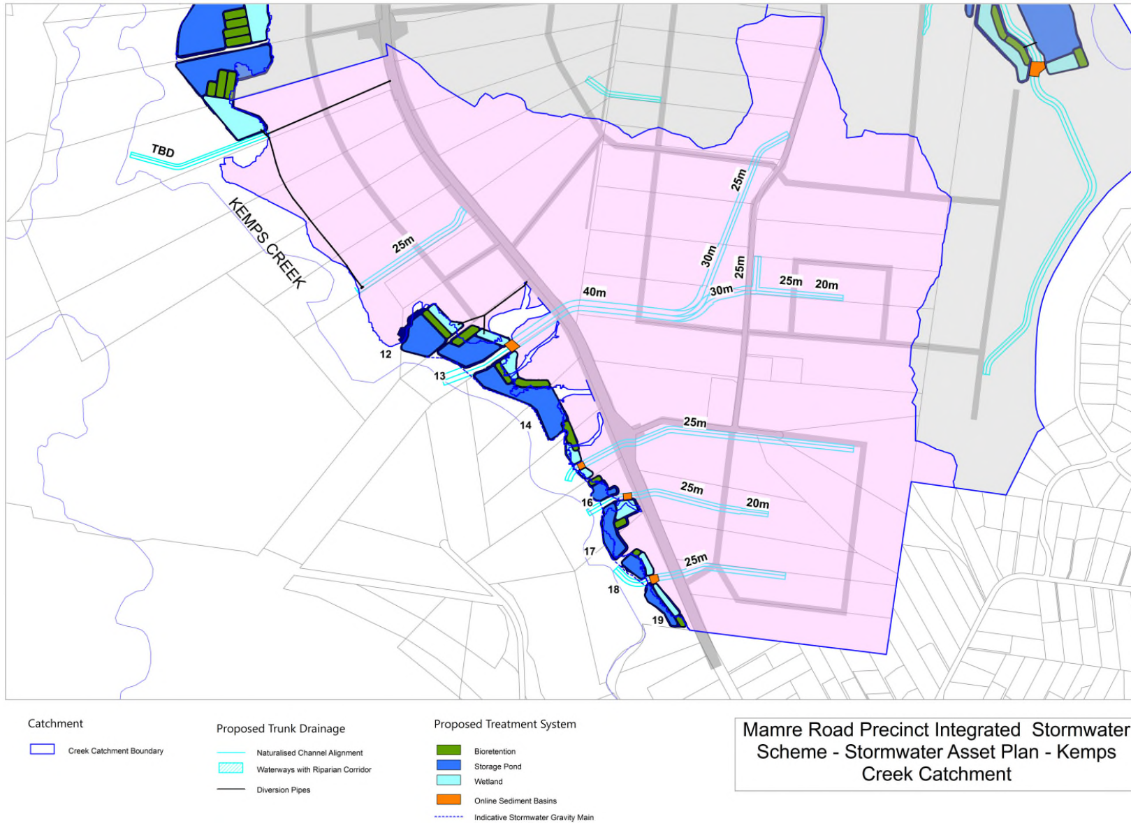
Figure 6.1.2 Stormwater assets in the Mamre Road Precinct Kemps Creek catchment
