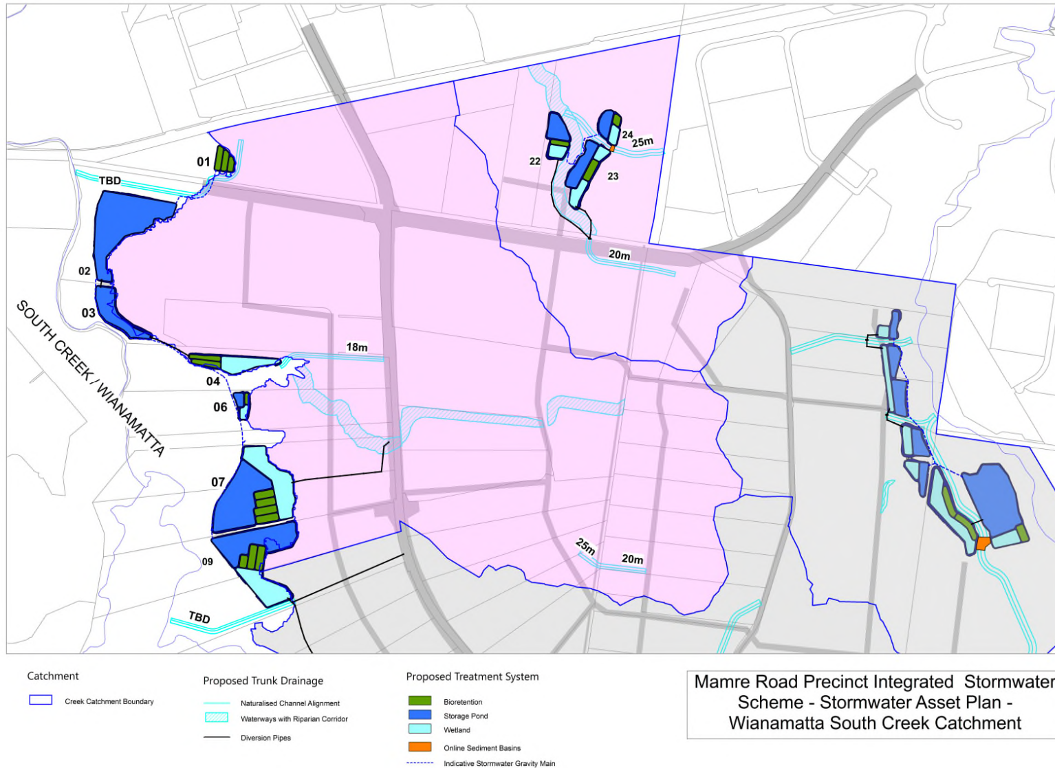
Figure 6.1.3 Stormwater assets in the Mamre Road South Creek catchment
