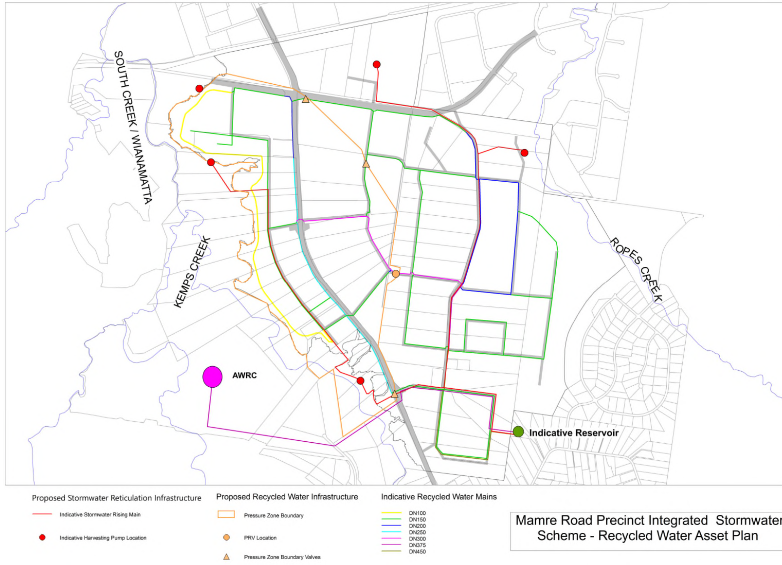
Figure 6-2 Recycled Water assets in Mamre Road Precinct
