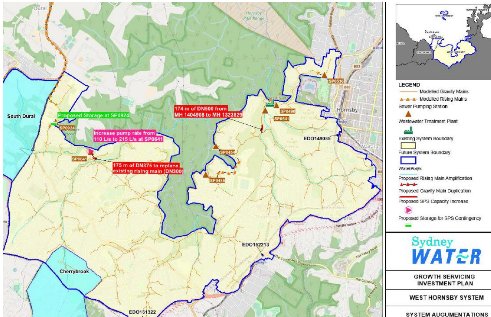
Figure 5-3 Investments needed to manage the impact of growth in the West Hornsby Wastewater System
