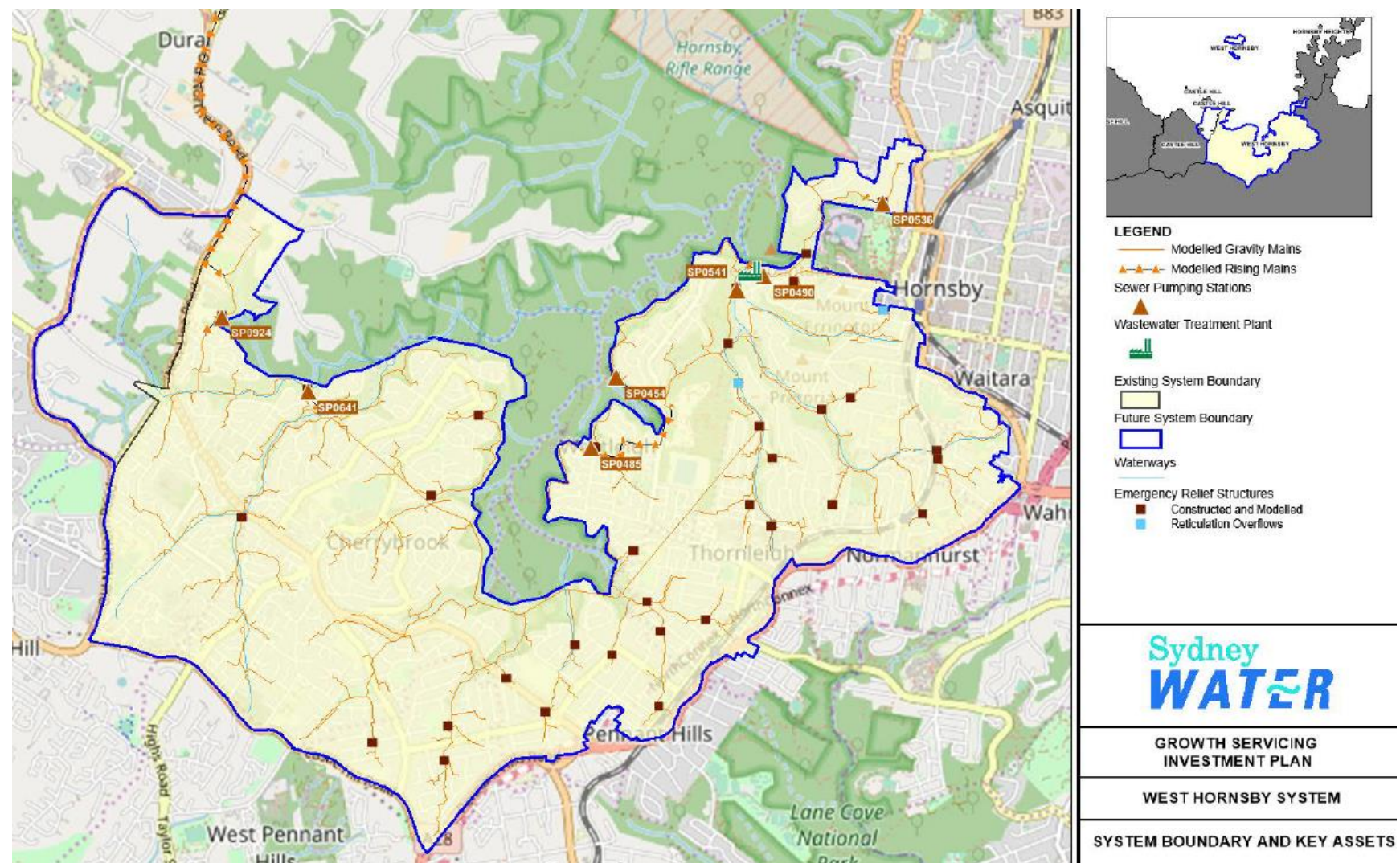
Figure 5-1 Major assets in the West Hornsby Wastewater System
